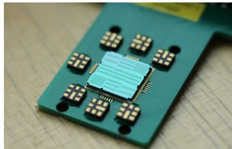
Nanoscale electrostatic drive (NED)-based ultrasound transducer (NEDMUT). © Fraunhofer IPMS
